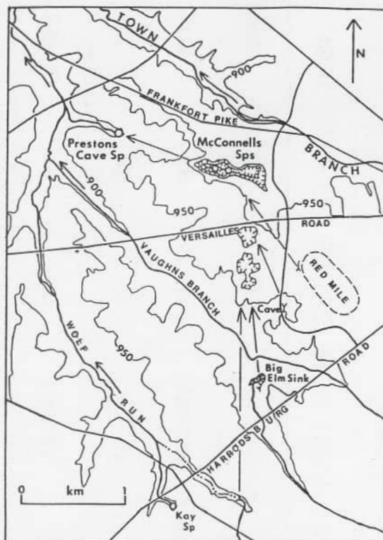
Generalized directions of flow in the Preston's Cave Spring groundwater basin.
