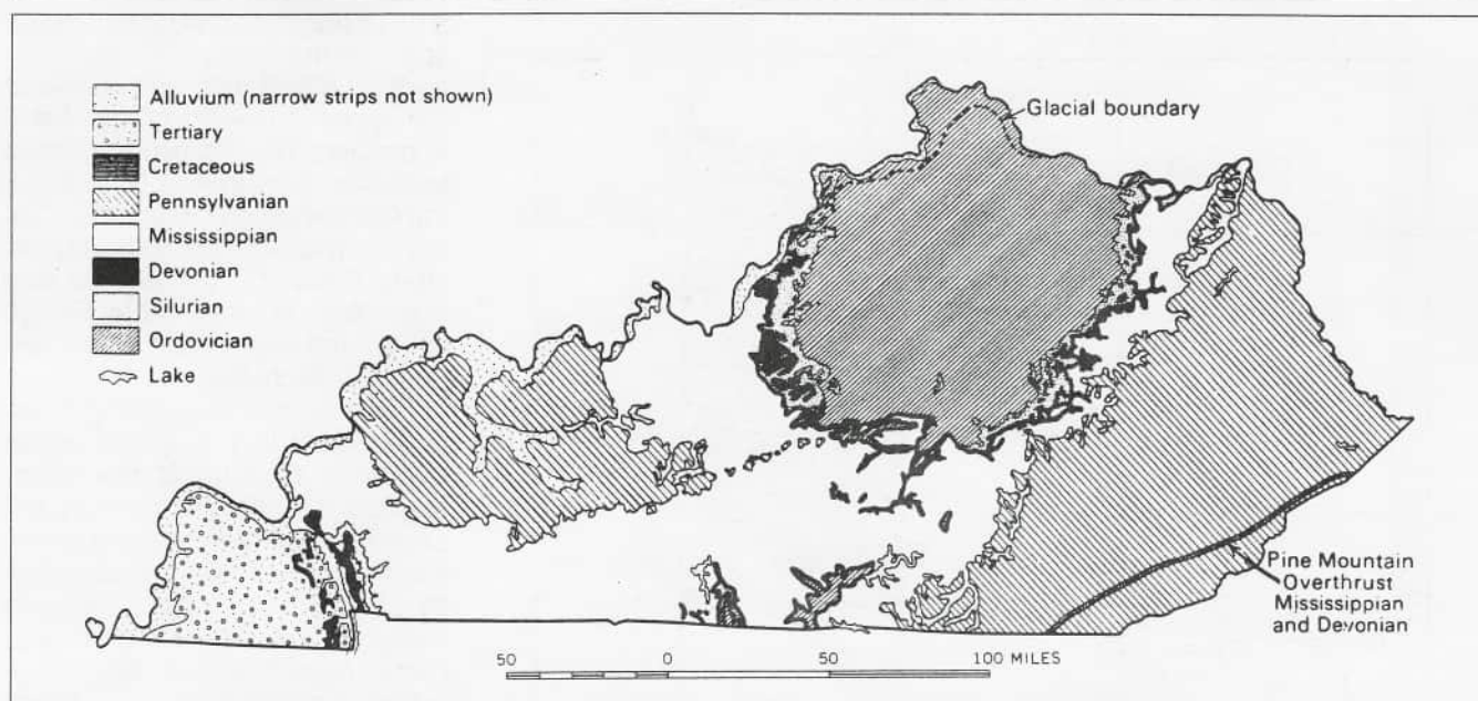
Figure 2. Geologic map showing the age of rock outcrops in Kentucky. From McFarlan, 1958, p. 5.
