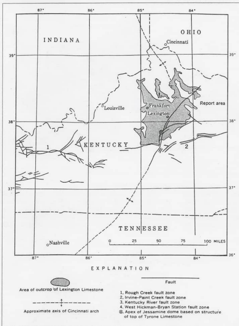
Figure 4. Index map showing the surface extent of the Lexington Limestone and major structural features. Faults are from the U.S. Geological Survey and American Association of Petroleum Geologists (1961); the area of outcrop of the Lexington Limestone is modified slightly from U.S. Geological Survey. From Cressman, 1973.
