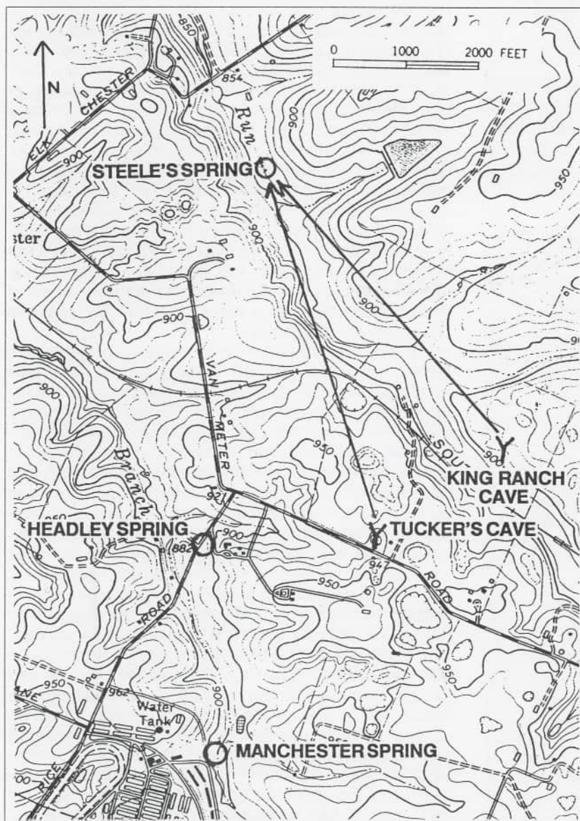
A portion of the Steele's Spring basins and adjacent springs
