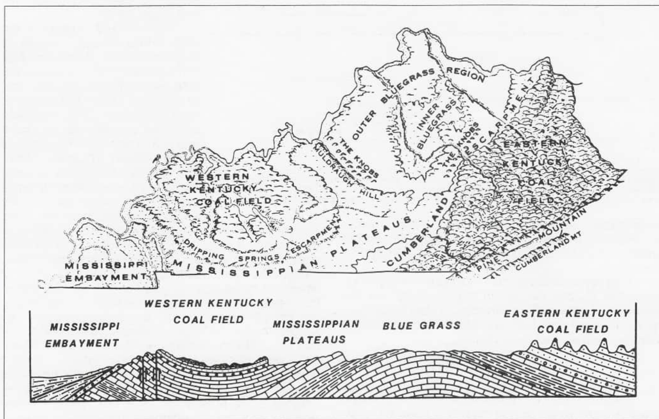
Figure 3. Physiographic map of Kentucky showing geomorphic regions and major escarpments. Generalized cross section depicts the structure of rock units from west to east across the state. From McGrain, 1983, p. 13.
