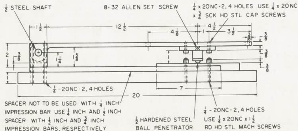
Fig. 1 Brinell Hardness Penetrator Assembly
