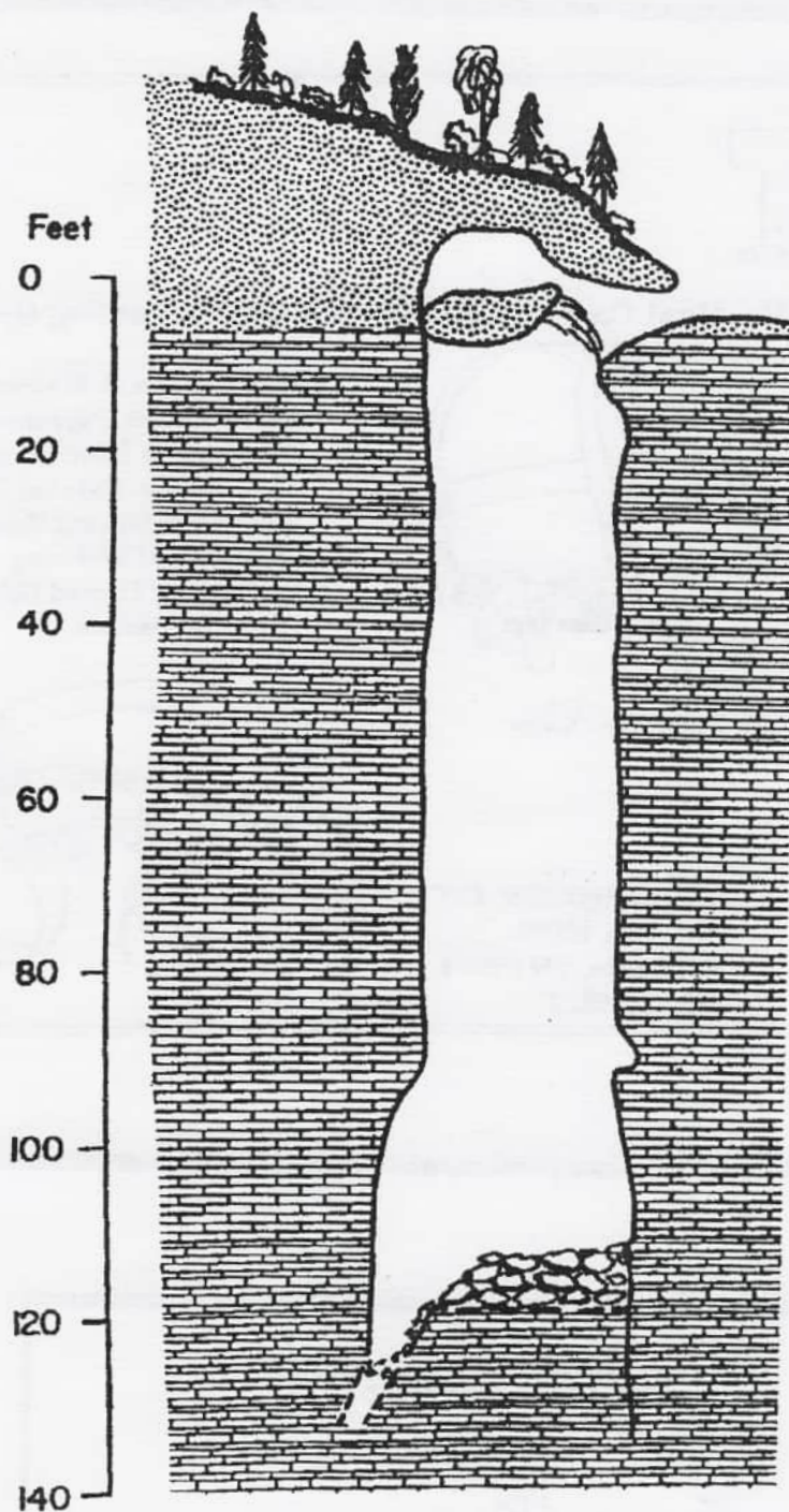
SINKS OF THE ROUNDSTONE PIT Rockcastle County, Kentucky
